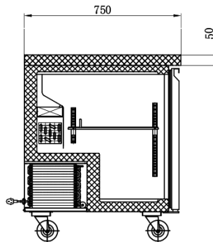
SECTION VIEW
